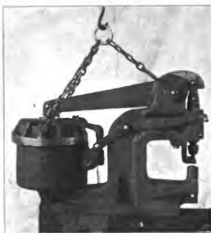
Fig. 4999. Portable Pneumatic Punch. Quincy, Manchester, Sargent Co.
